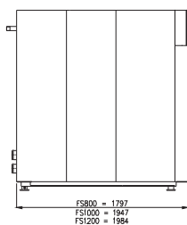
SIDE FS800 1000 1200
